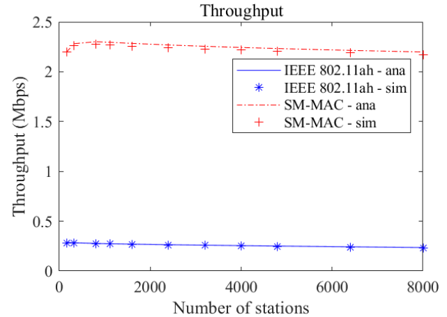
Fig. 13: Throughput versus the number of stations.
